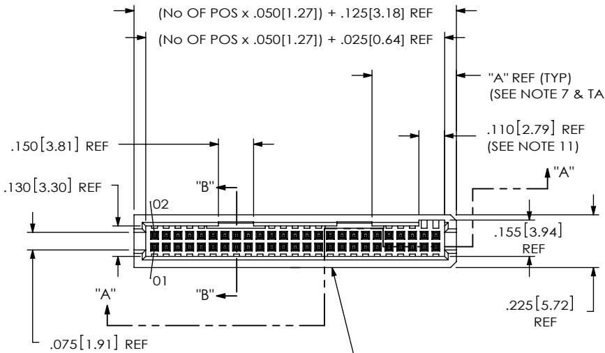
FIG. 1 -01: THROUGH HOLE
